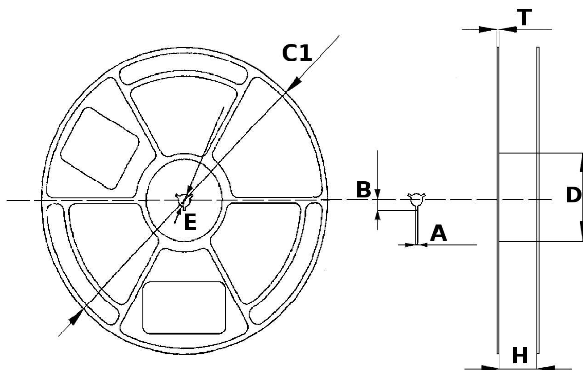
Figure 16 - Reel Specifications
